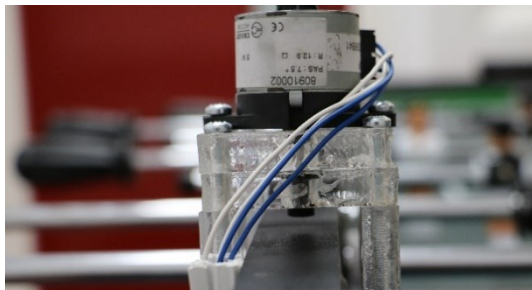
Figure 3: One of the acrylic clamps used to increase the friction on the users' rods. The clamp has a linear actuator installed on the top connected with a screw. Hitting the red plate sends signals to the actuator, which causes the screw to pull the clamp upwards, making harder to move the rods.
